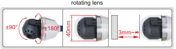
±90° rotation in radial direction, ±180° rotation in axial direction diameter (ØD) focus distance (F)
