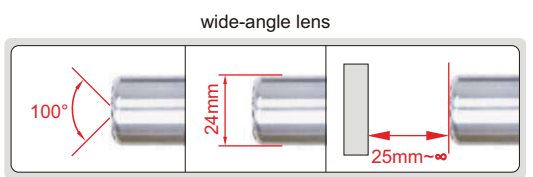
angle of view (θ) diameter (ØD) focus distance (F)
